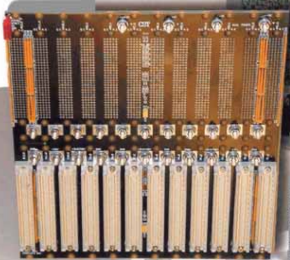
Custom backplane design and assembly
